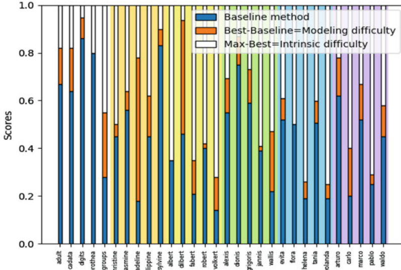
Fig. 10.5 Difficulty of tasks in the 2015/2016 challenge. We consider two indicators of task difficulty (dataset, metric, and time budget are factored into the task): intrinsic difficulty (estimated by the performance of the winners) and modeling difficulty (difference between the performance of the winner and a baseline method, here Selective Naive Bayes (SNB)). The best tasks should have a relatively low intrinsic difficulty and a high modeling difficulty to separate participants well
