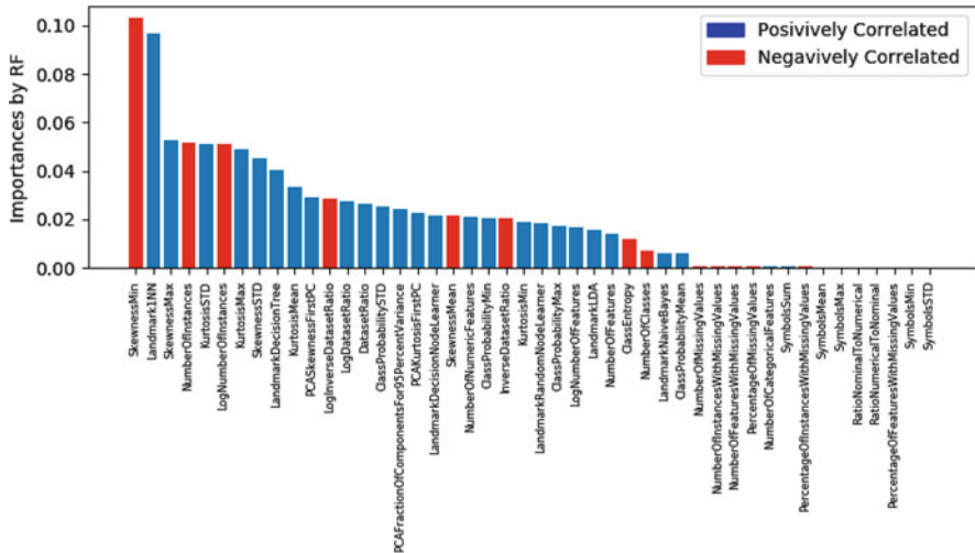
Fig. 10.7 Meta-feature GINI importances most predictive of dataset intrinsic difficulty (2015/2016 challenge data). Meta-feature GINI importances are computed by a random forest regressor, trained to predict the highest participant leaderboard score using meta-features of datasets. Description of these meta-features can be found in Table 1 of the supplementary material of [25]. Blue and red colors respectively correspond to positive and negative correlations (Pearson correlations between meta features and score medians)
